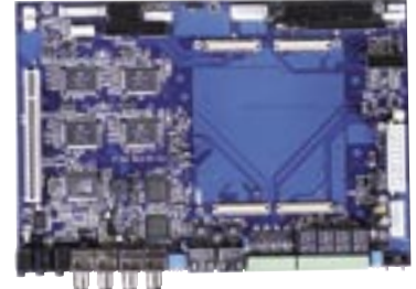
ETX-DB-DVR1 ETX Baseboard with 4 Capture Engine CF II, Dual LAN, Audio & D I/O
