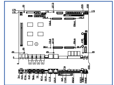
ETX-DB-DVR1 ETX Baseboard with 4 Capture Engine CF II, Dual LAN, Audio & D I/O
