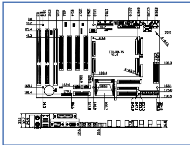
ETX-DB-7SR Full Function ETX Baseboard with LCD/CRT VGA, Audio, DOC, CF II & D I/O
