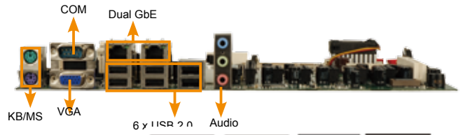
NVIDIA MCP55Pro server-grade chipset
