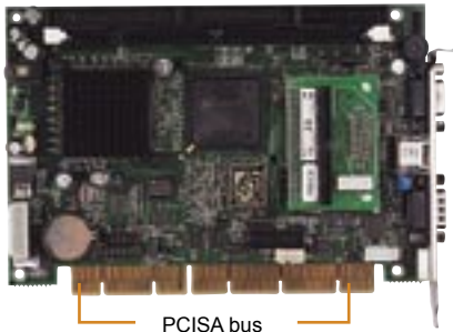
PCISA bus
